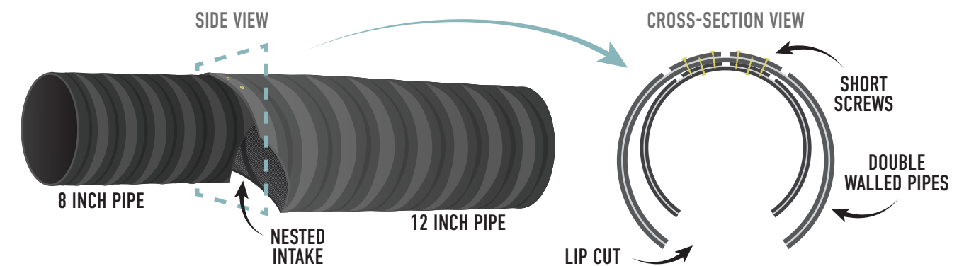
Figure 4. Nested pipe configuration used when constructing a dual-intake pond leveler.
