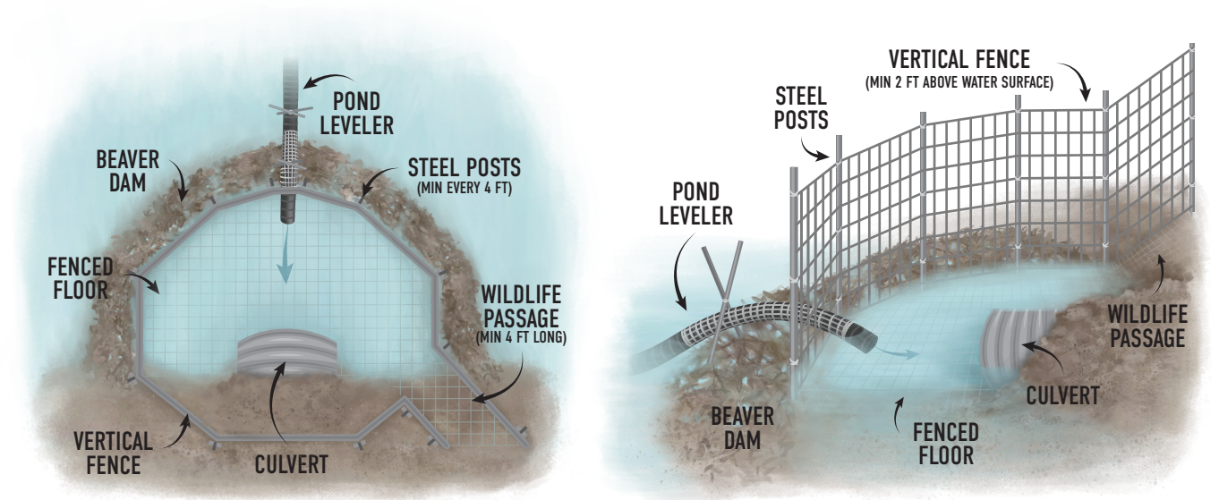
Figure 10. The combination of an anchor fence and pond leveler to create a pipe and fence culvert protection system shown from above (left) and side (right).
