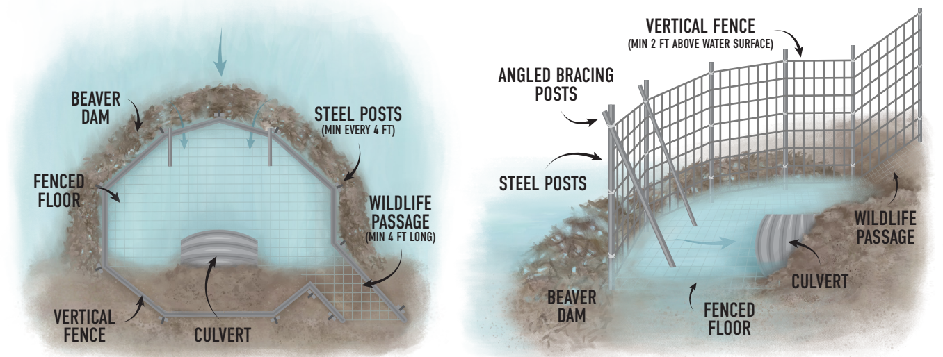
Figure 9. Standard anchor fence shown from above (left) and side (right).
